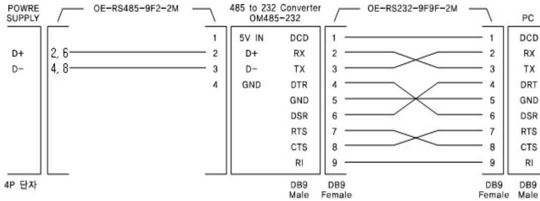
485 to 232 Converter
